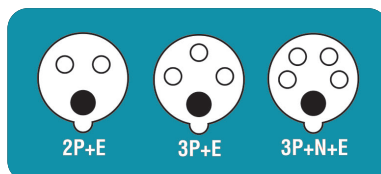
Socket Front View
